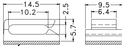
3M DOUBLE ADHESIVE TAPE (THICKNESS 1.1mm)
