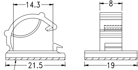
3M DOUBLE ADHESIVE TAPE (THICKNESS 1.1mm)
